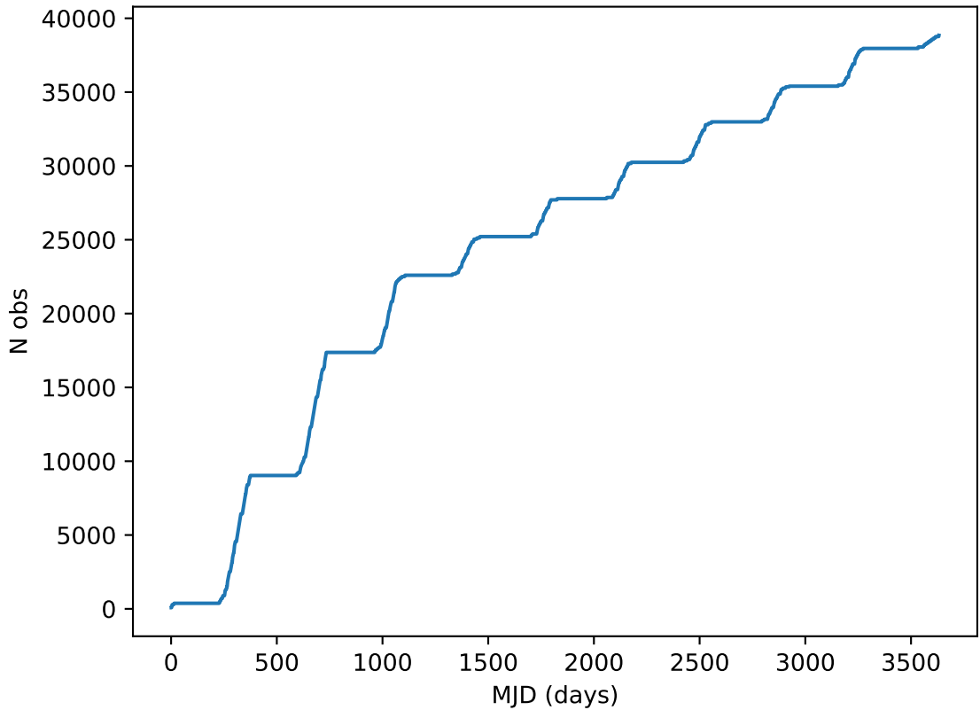
ddf_acor_sf30_lsf40_lsr20_v3.4_10yrs all bands: DD: COSMOS Cumulative NVisits
