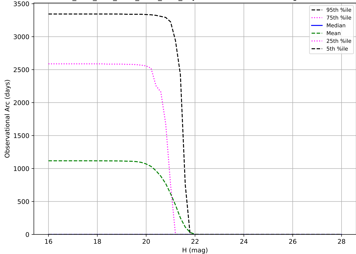
ddf_acor_sf30_lsf40_lsr10_v3.4_10yrs: Observational Arc Length Vatira
