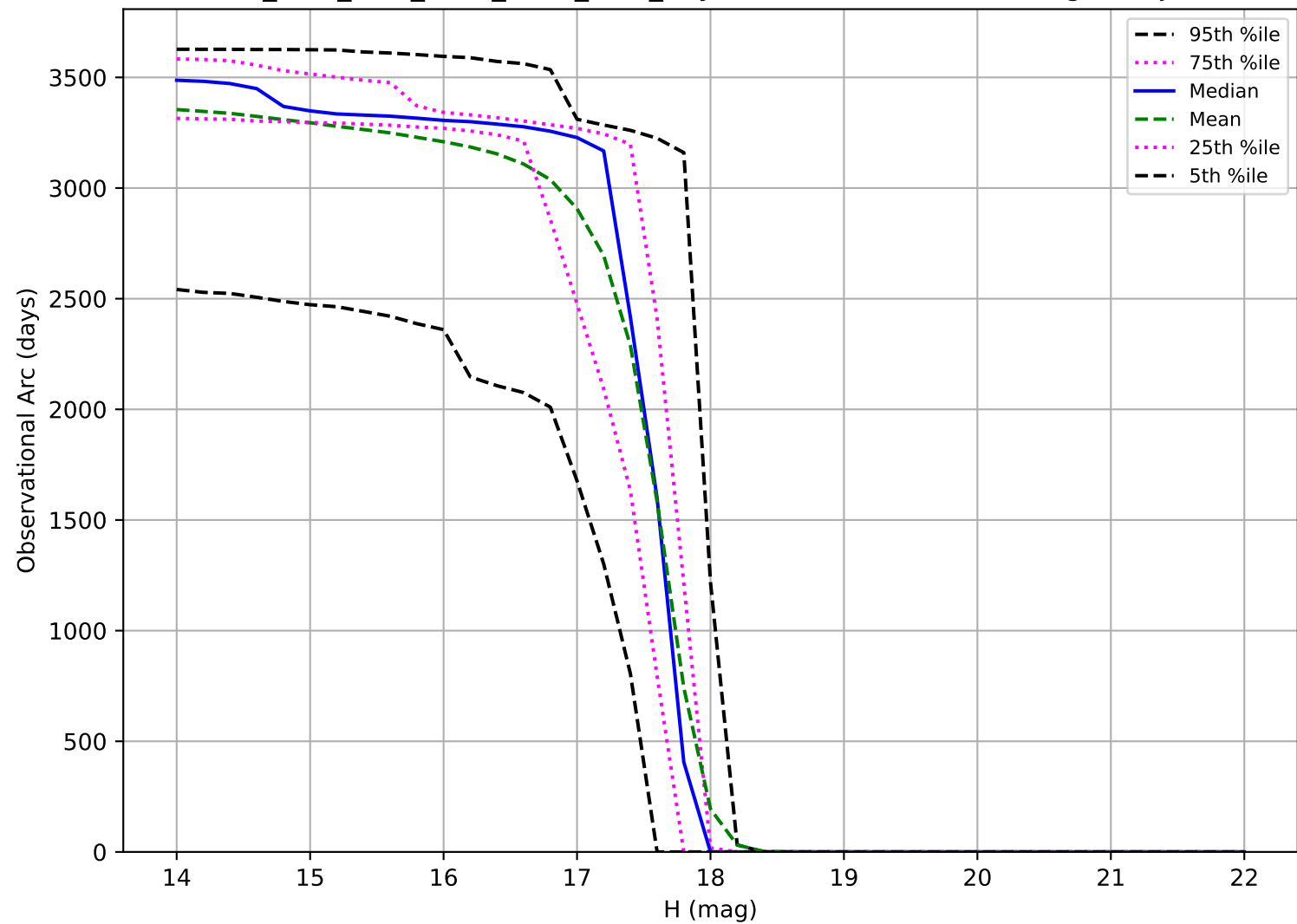
ddf_acor_sf30_lsf40_lsr10_v3.4_10yrs: Observational Arc Length Trojan
