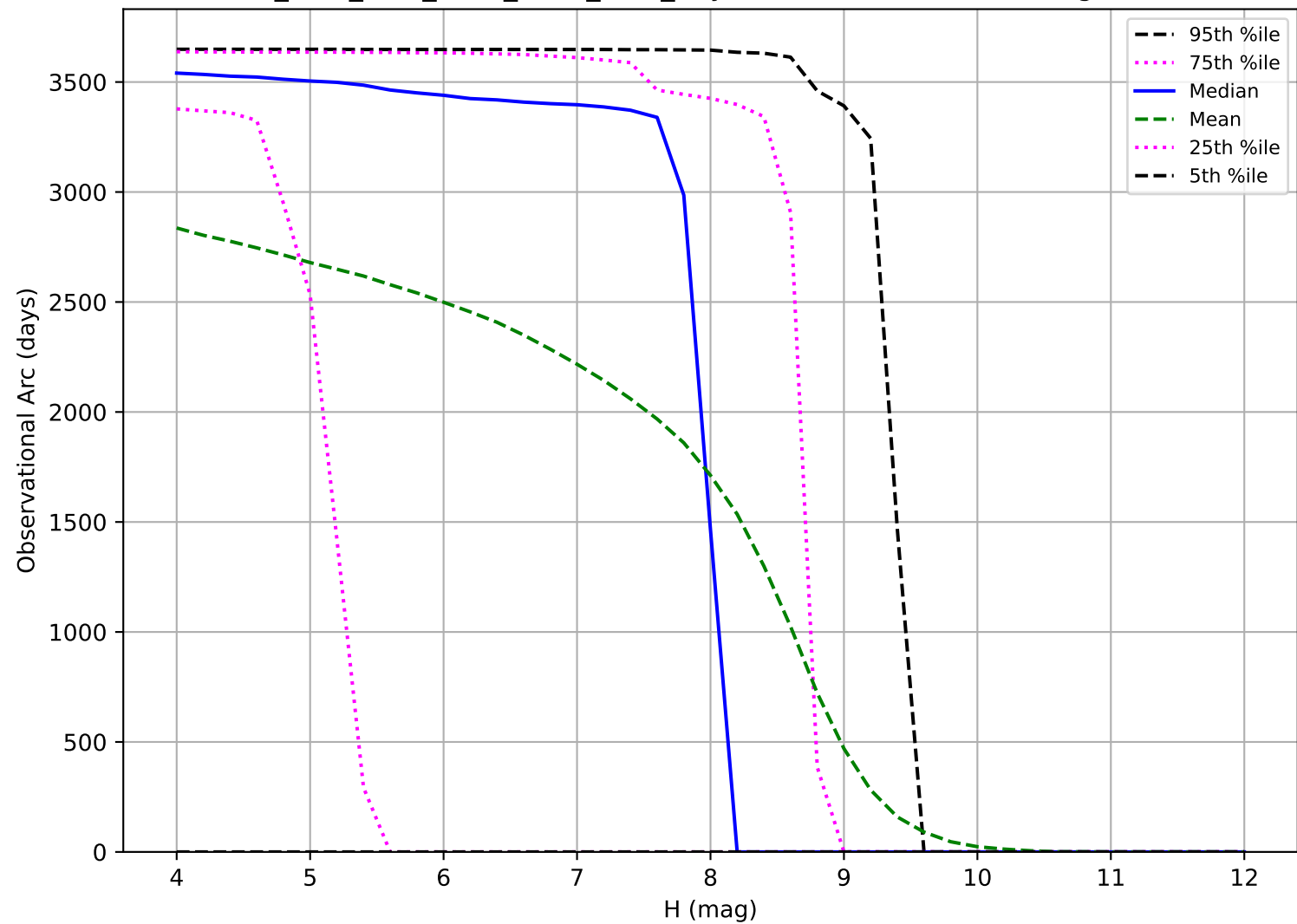
ddf_acor_sf30_Isf40_Isr10_v3.4_10yrs: Observational Arc Length TNO
