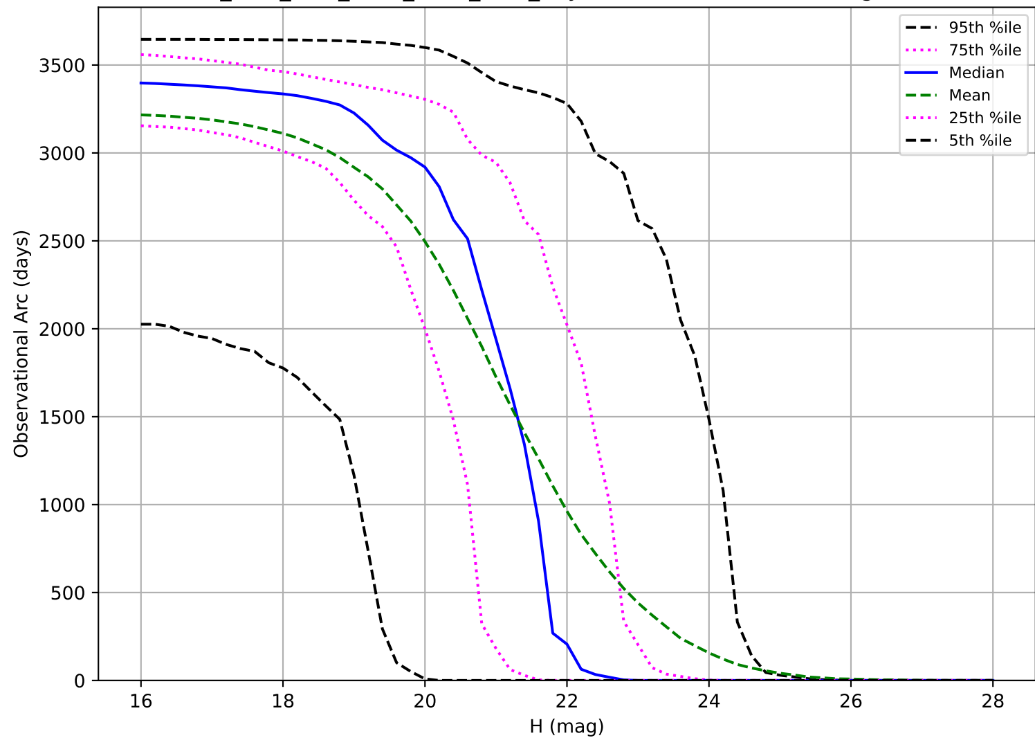
ddf_acor_sf30_lsf40_lsr10_v3.4_10yrs: Observational Arc Length PHA
