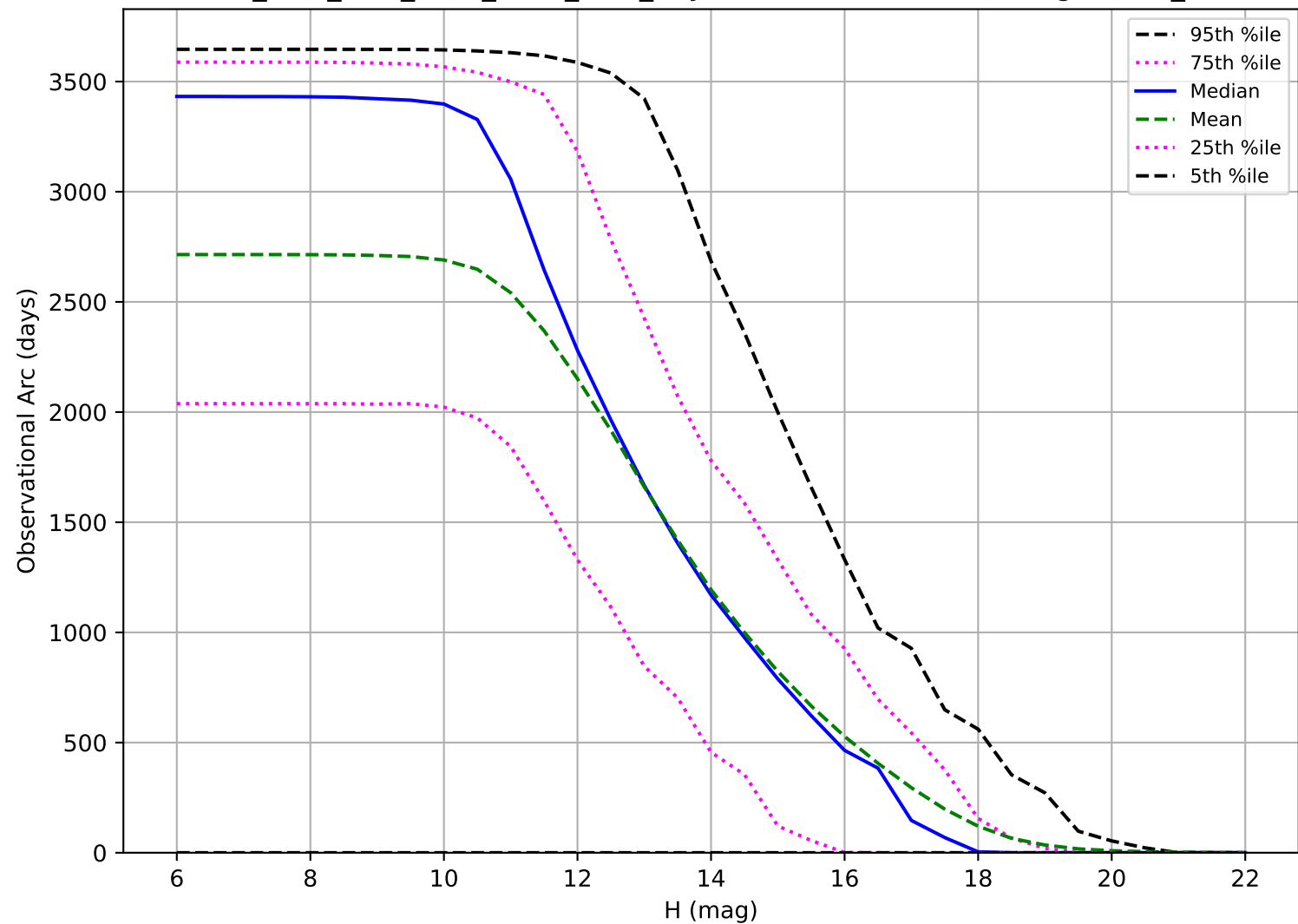
ddf_acor_sf30_lsf40_lsr10_v3.4_10yrs: Observational Arc Length OCC_r5
