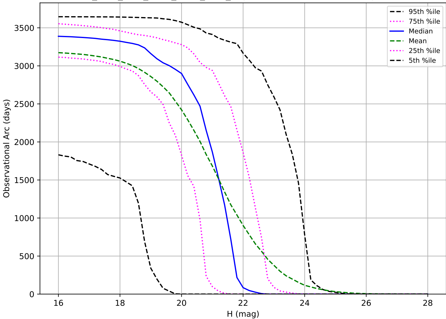
ddf_acor_sf30_lsf40_lsr10_v3.4_10yrs: Observational Arc Length NEO
