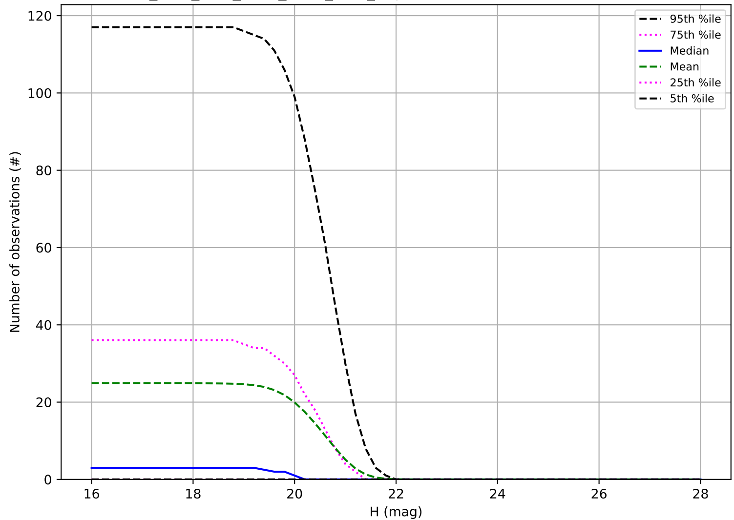
ddf_acor_sf30_lsf40_lsr10_v3.4_10yrs: Number of observations Vatira
