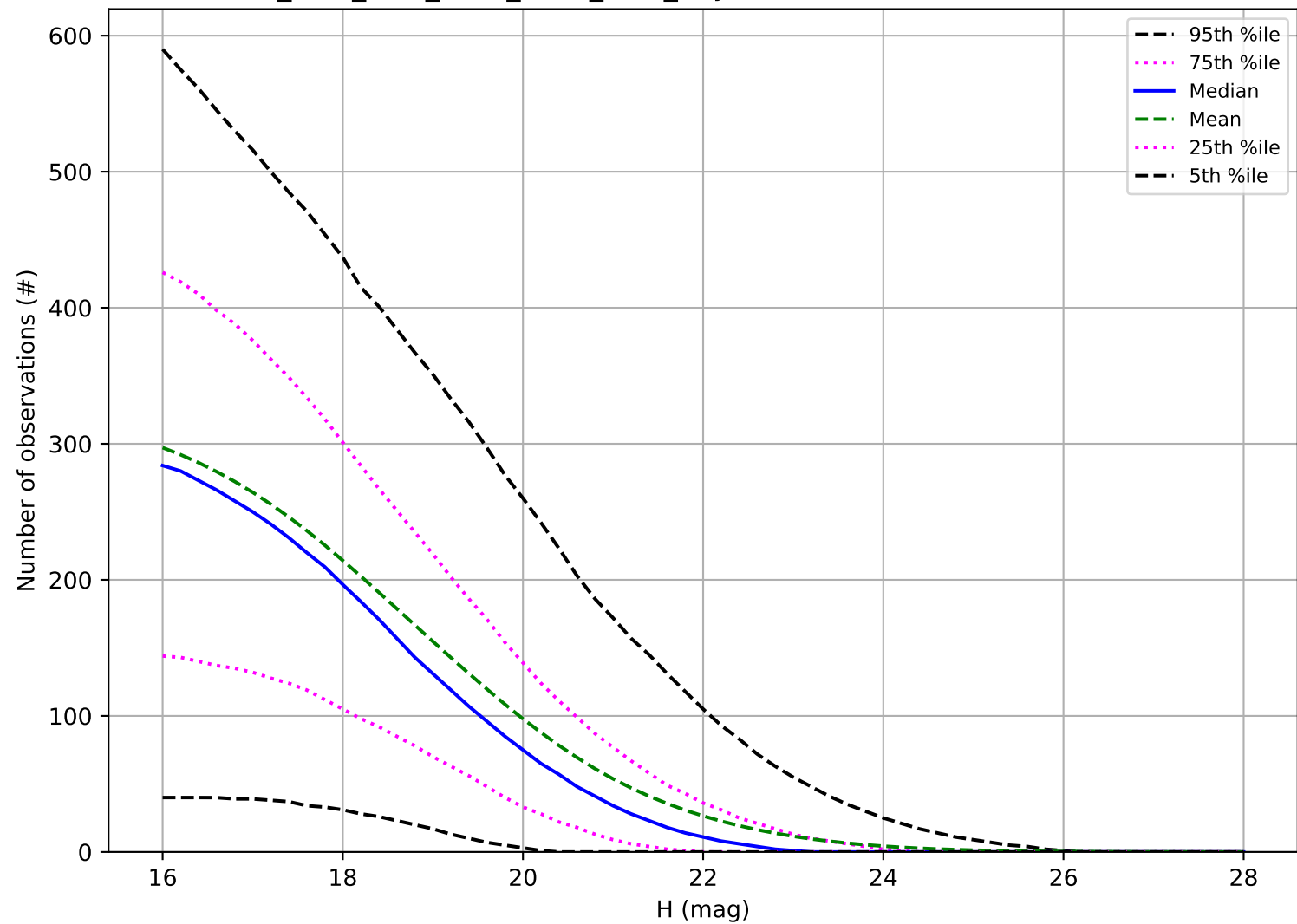
ddf_acor_sf30_lsf40_lsr10_v3.4_10yrs: Number of observations PHA
