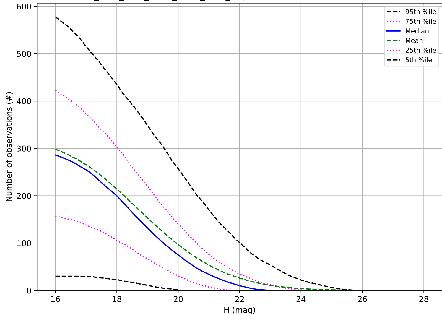
ddf_acor_sf30_lsf40_lsr10_v3.4_10yrs: Number of observations NEO
