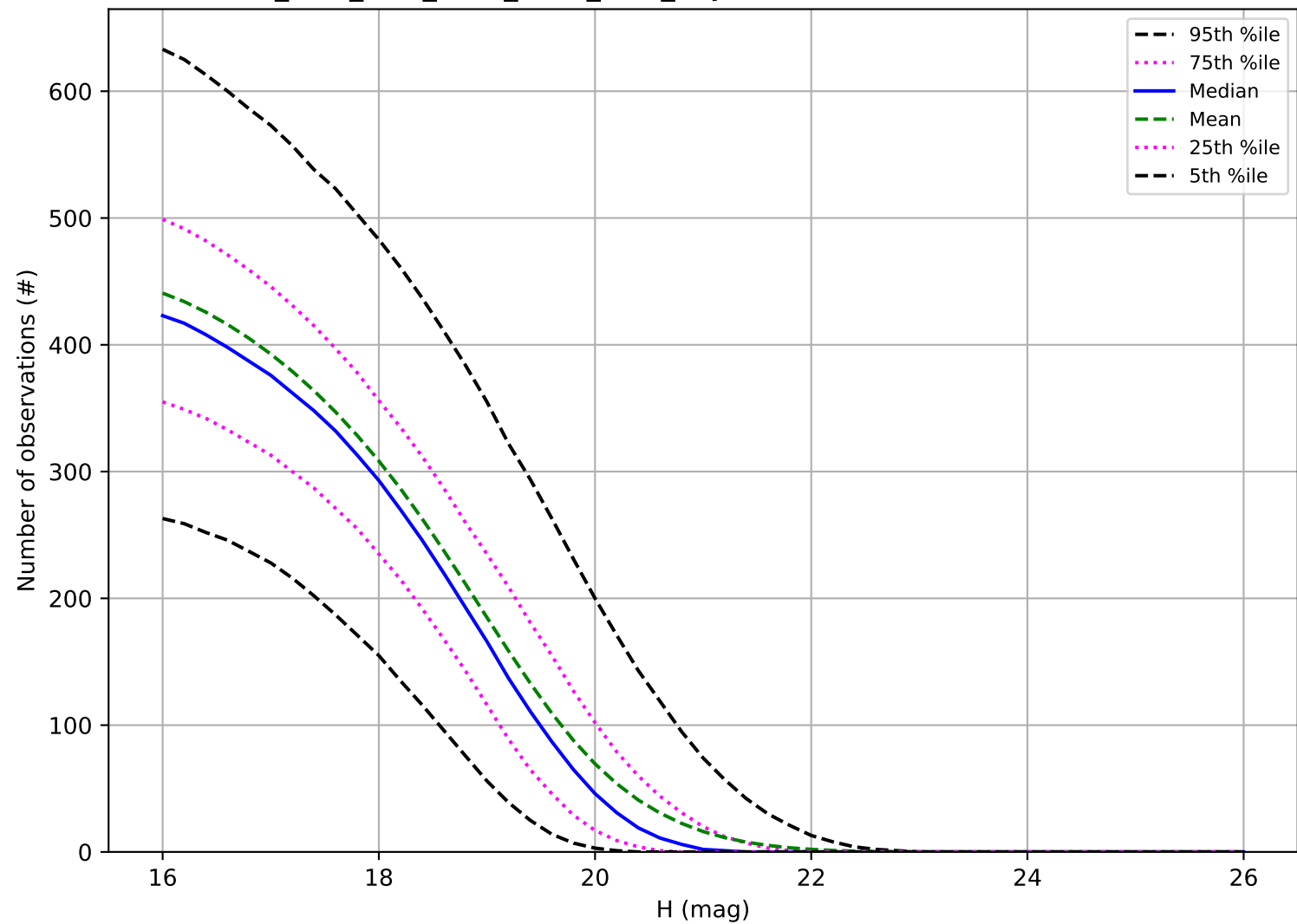
ddf_acor_sf30_lsf40_lsr10_v3.4_10yrs: Number of observations MBA
