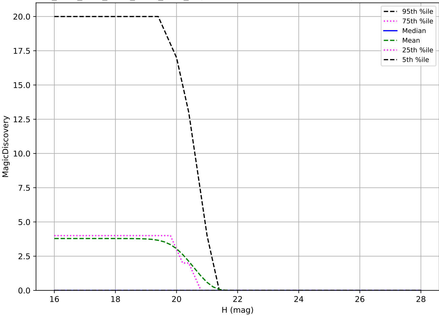
ddf_acor_sf30_lsf40_lsr10_v3.4_10yrs: Vatra 6 detections in 60 nights detection loss
