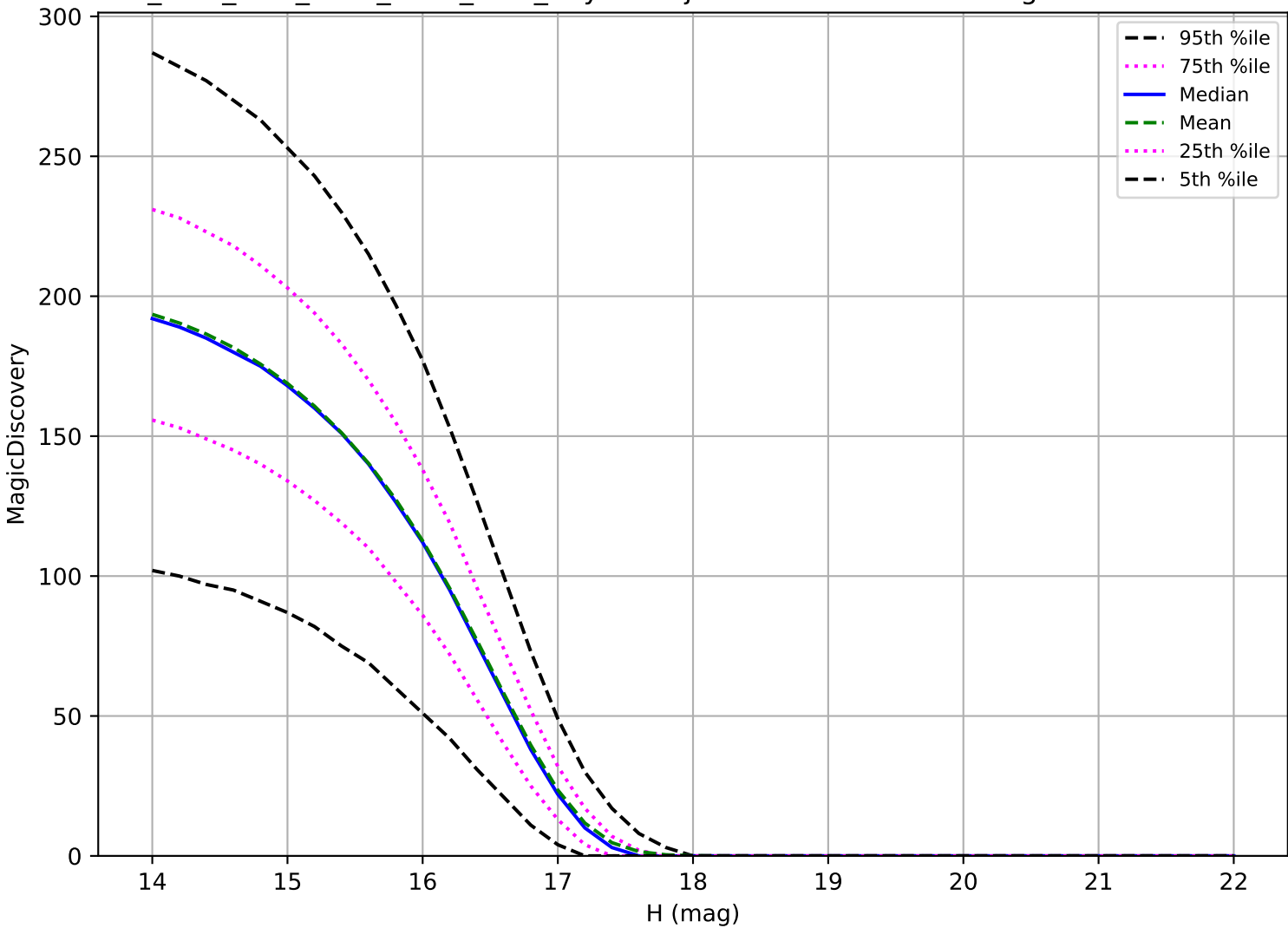
ddf_acor_sf30_lsf40_lsr10_v3.4_10yrs: Trojan 6 detections in 60 nights detection loss
