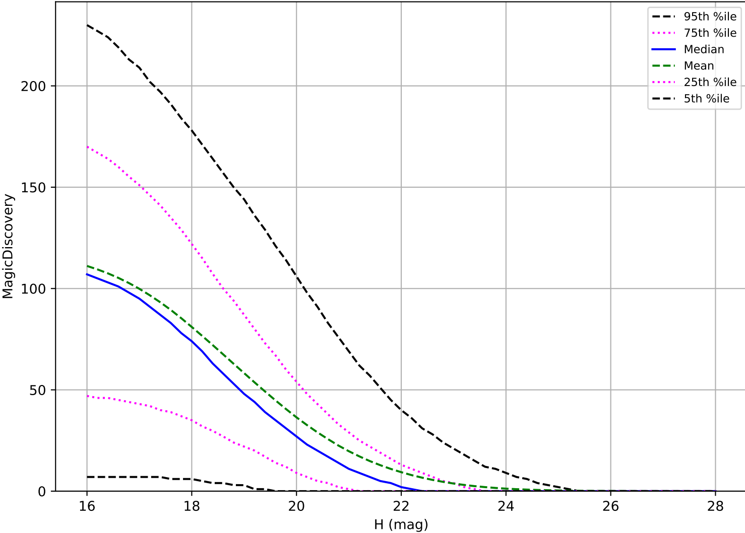
ddf_acor_sf30_lsf40_lsr10_v3.4_10yrs: PHA 6 detections in 60 nights detection loss
