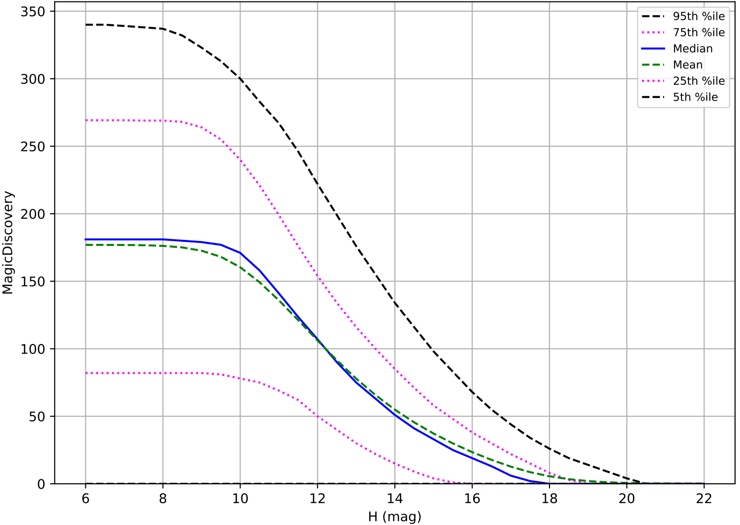
ddf_acor_sf30_lsf40_lsr10_v3.4_10yrs: OCC_r5 6 detections in 60 nights detection loss
