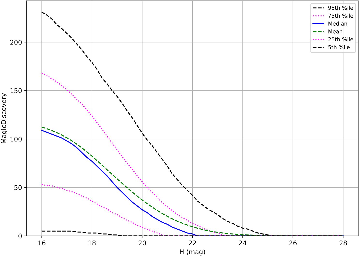
ddf_acor_sf30_lsf40_lsr10_v3.4_10yrs: NEO 6 detections in 60 nights detection loss
