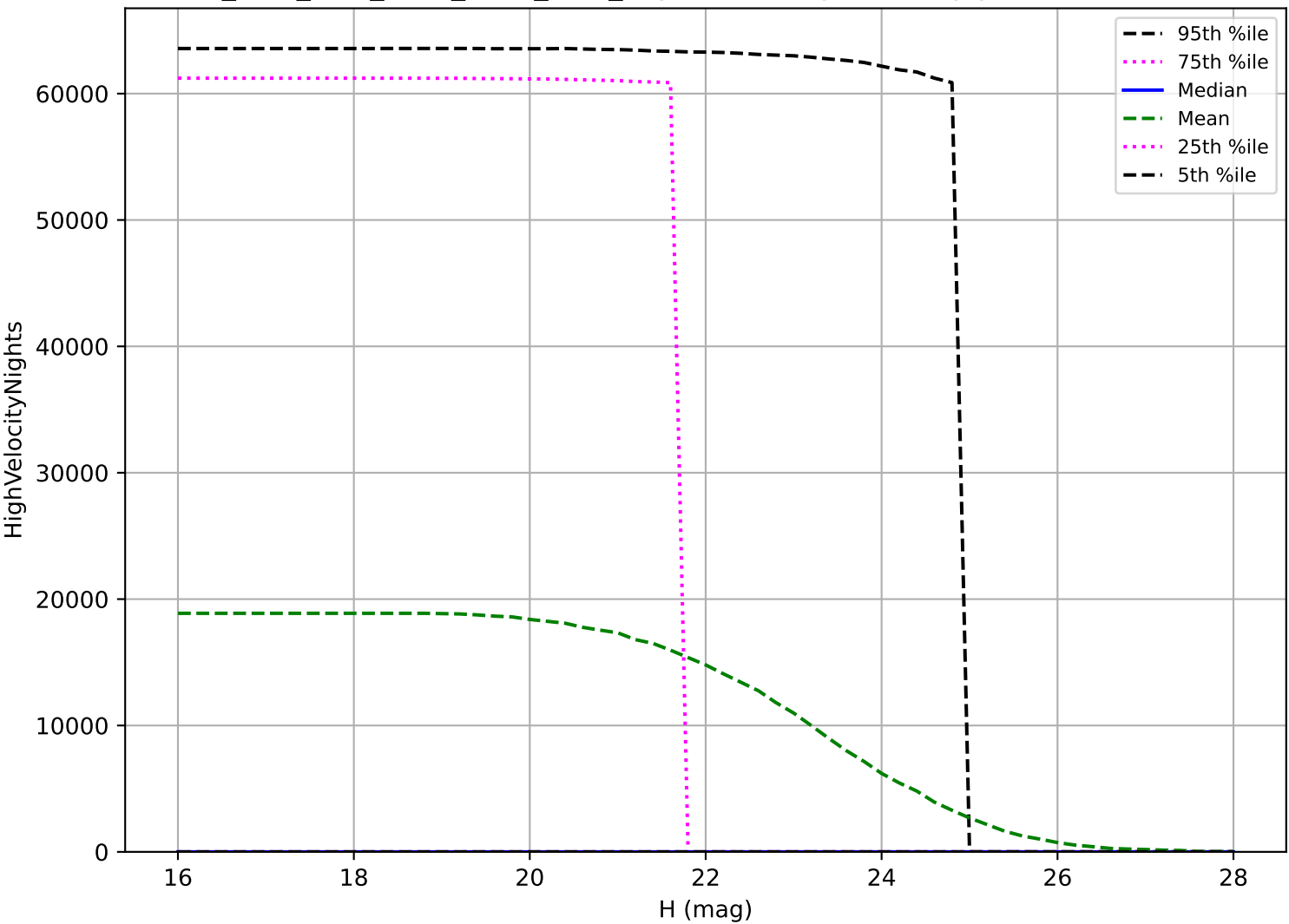
ddf_acor_sf30_lsf40_lsr10_v3.4_10yrs: NEO High velocity pair detection loss
