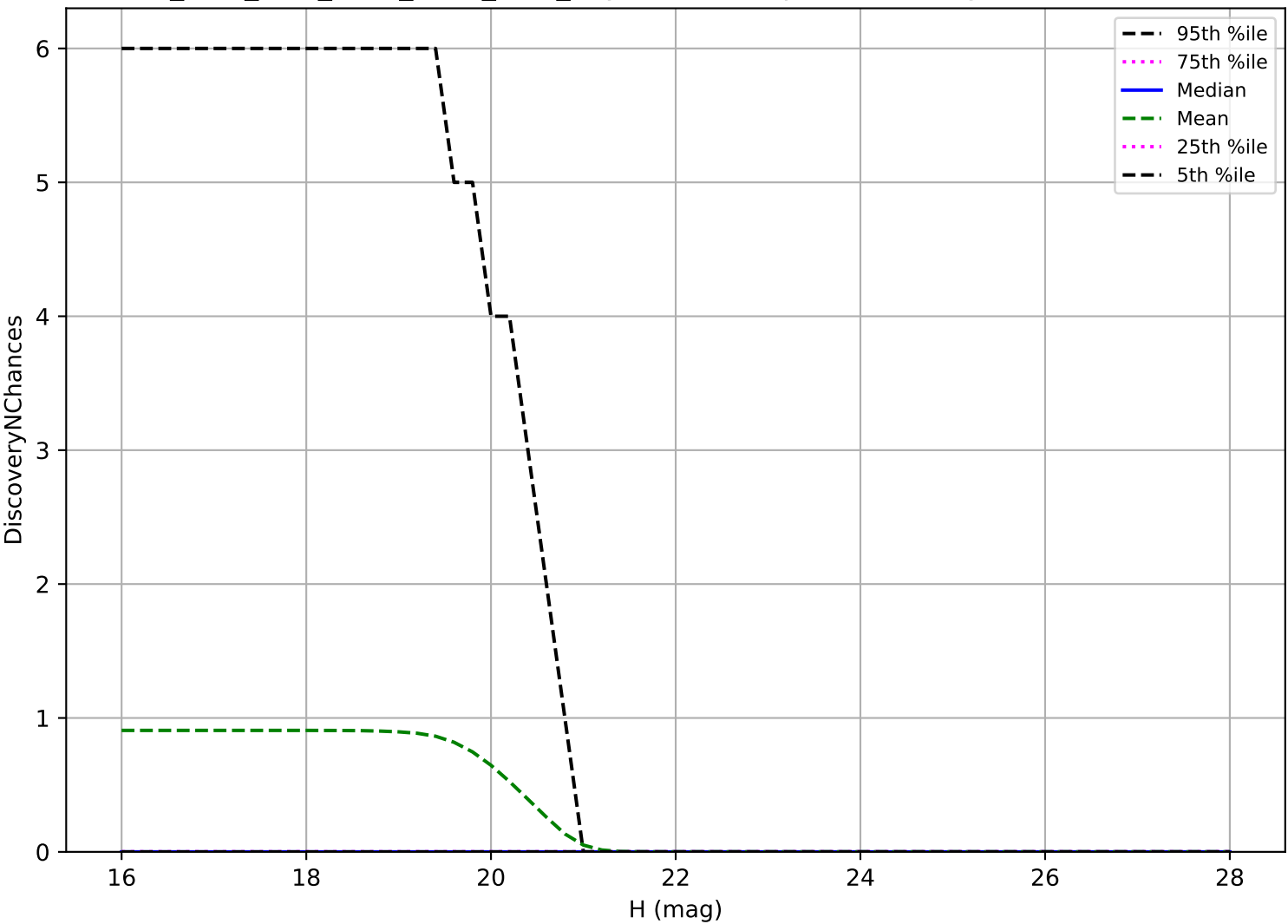
ddf_acor_sf30_lsf40_lsr10_v3.4_10yrs: Vatira 3 pairs in 15 nights detection loss
