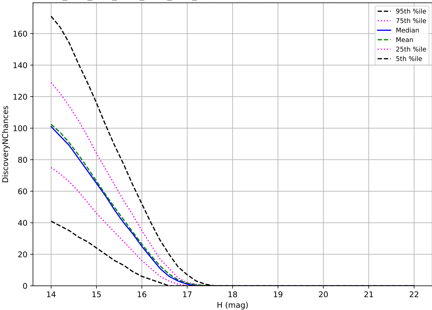
ddf_acor_sf30_lsf40_lsr10_v3.4_10yrs: Trojan 3 pairs in 15 nights detection loss
