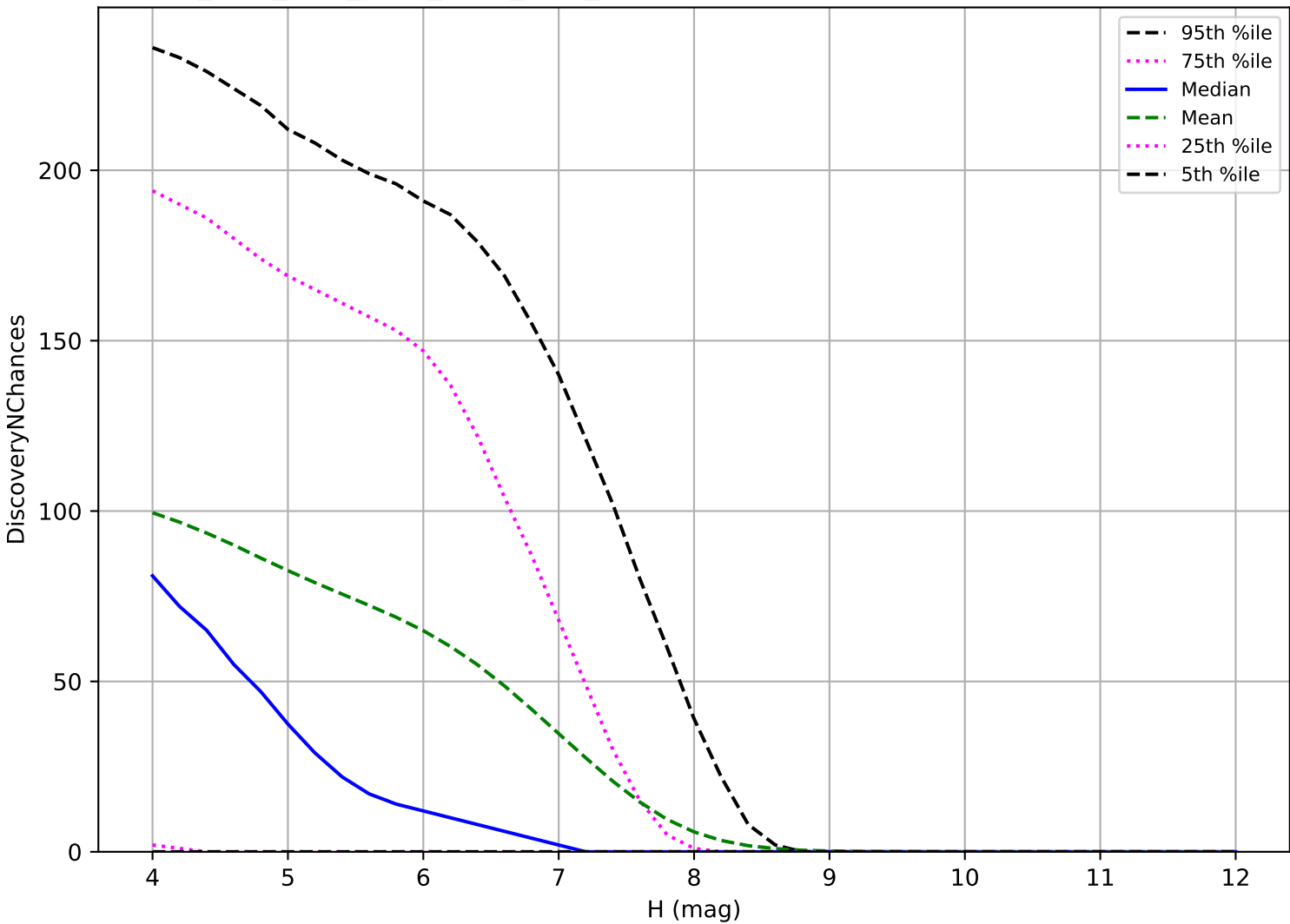
ddf_acor_sf30_lsf40_lsr10_v3.4_10yrs: TNO 3 pairs in 15 nights detection loss
