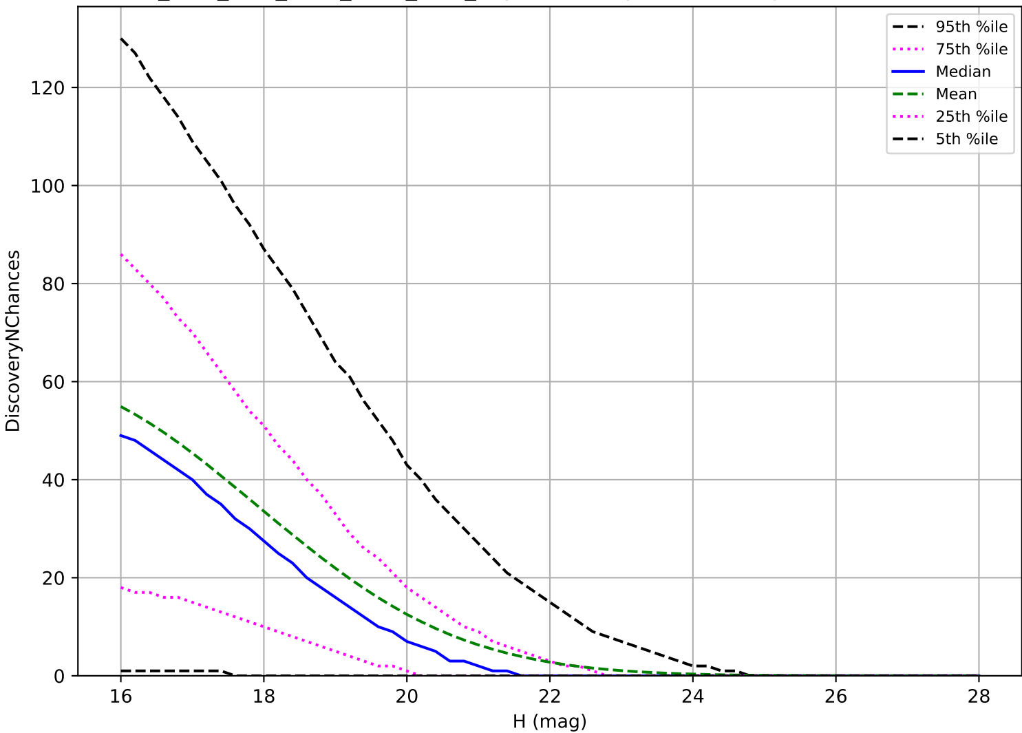
ddf_acor_sf30_lsf40_lsr10_v3.4_10yrs: PHA 3 pairs in 15 nights detection loss
