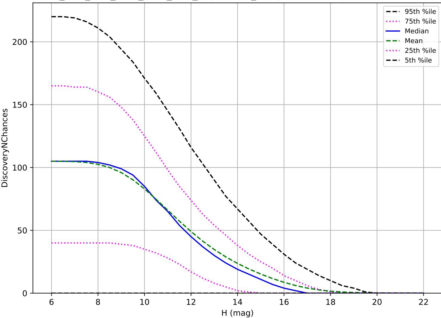
ddf_acor_sf30_lsf40_lsr10_v3.4_10yrs: OCC_r5 3 pairs in 15 nights detection loss
