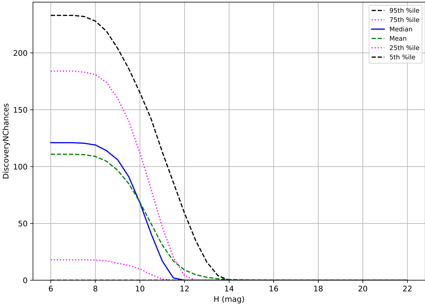
ddf_acor_sf30_lsf40_lsr10_v3.4_10yrs: OCC_r20 3 pairs in 15 nights detection loss
