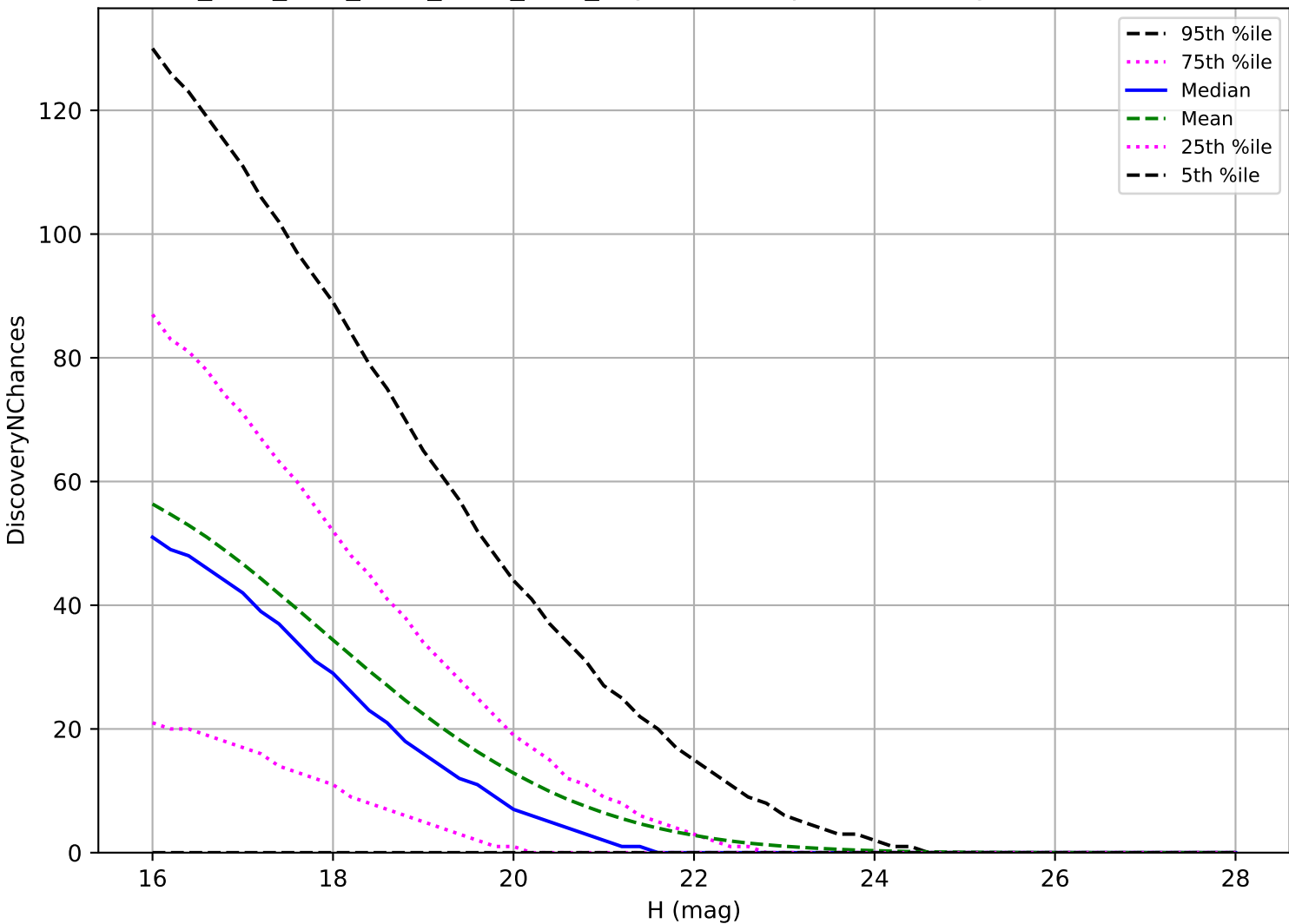
ddf_acor_sf30_lsf40_lsr10_v3.4_10yrs: NEO 3 pairs in 15 nights detection loss
