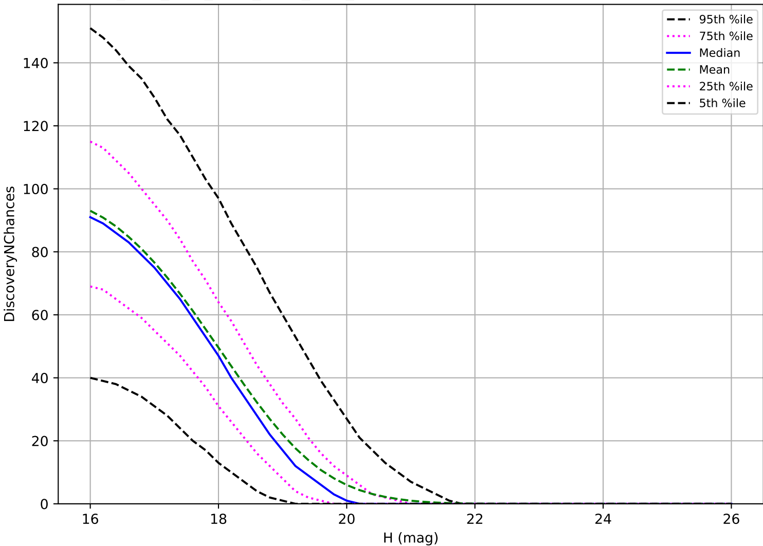
ddf_acor_sf30_lsf40_lsr10_v3.4_10yrs: MBA 3 pairs in 15 nights detection loss
