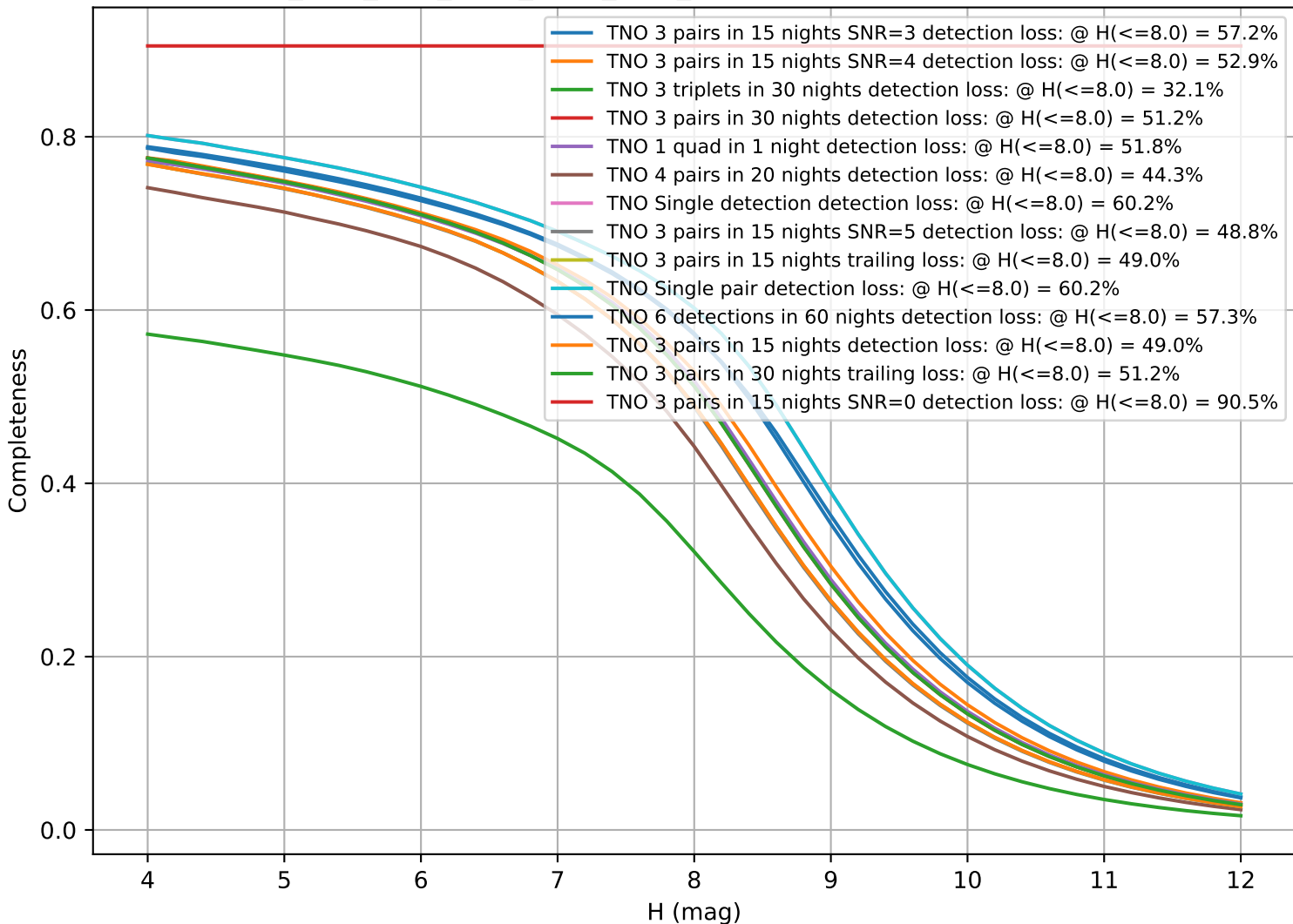
ddf_acor_sf30_lsf40_lsr10_v3.4_10yrs: CumulativeCompleteness
