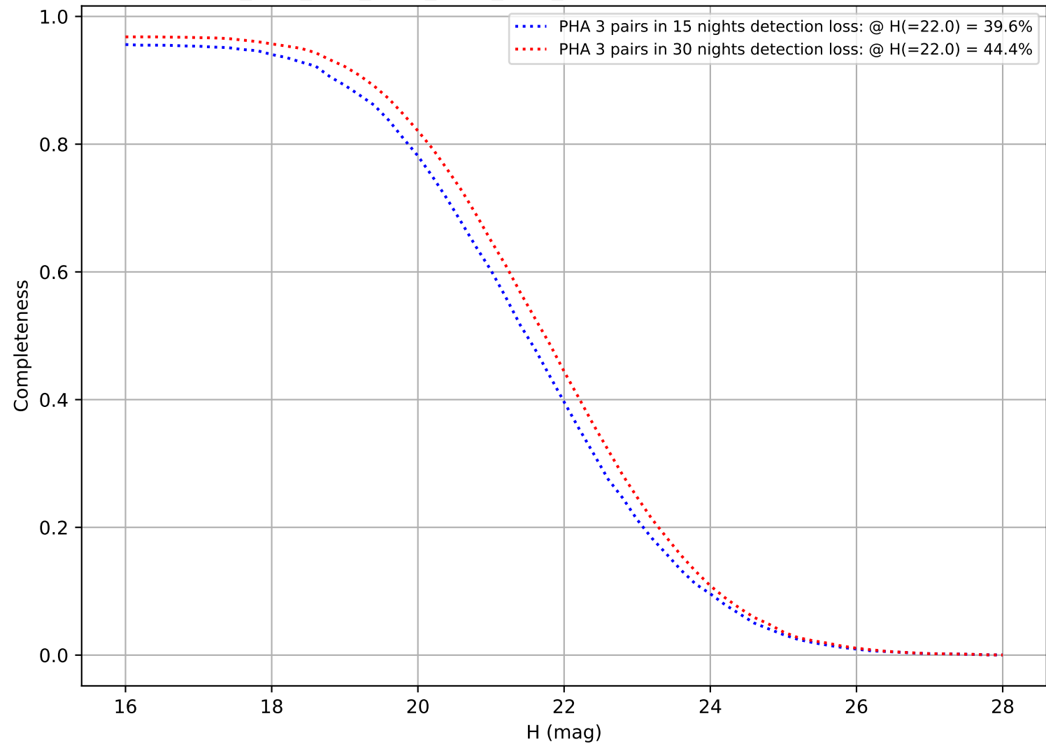
ddf_acor_sf30_lsf40_lsr10_v3.4_10yrs: DifferentialCompleteness
