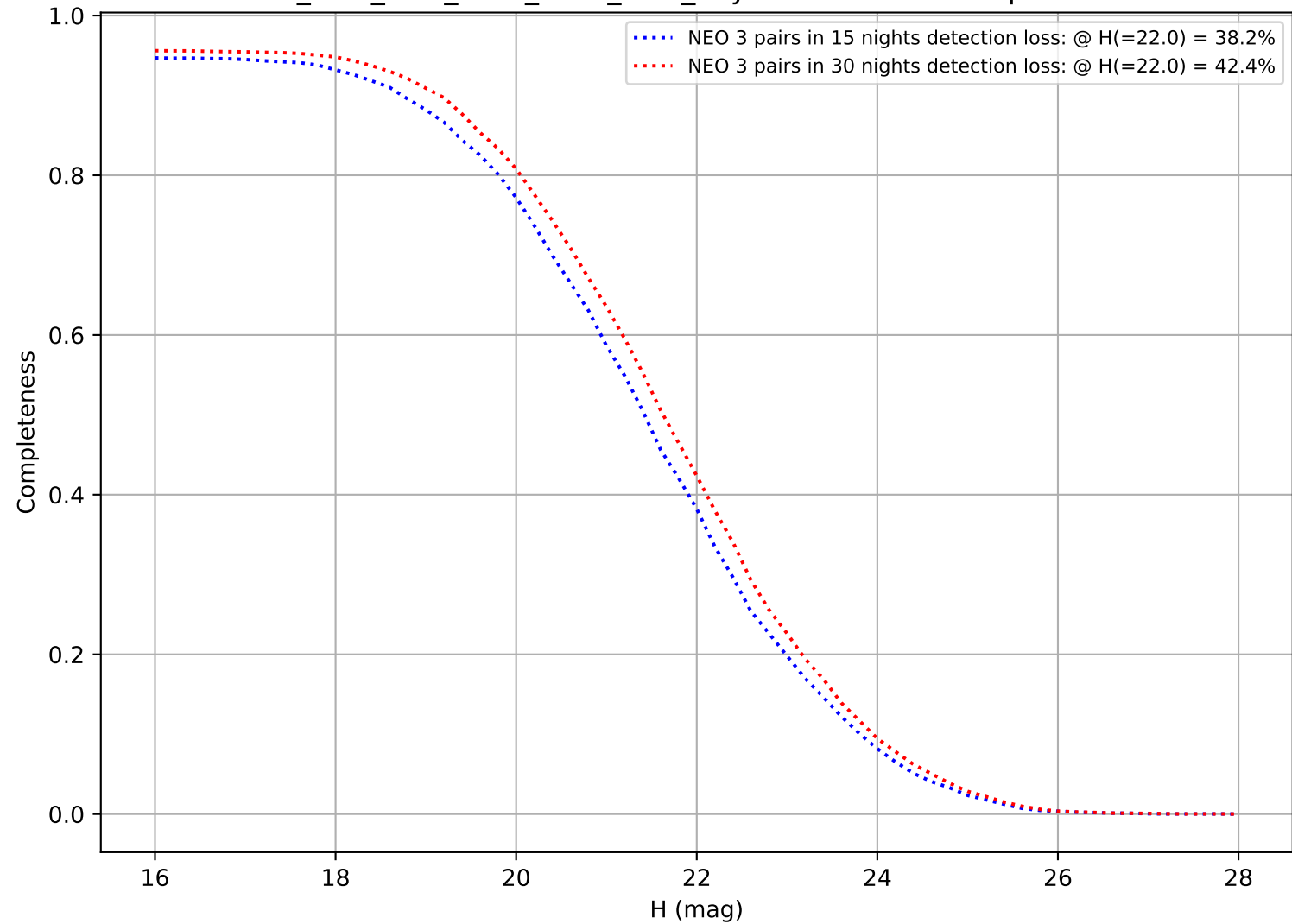
ddf_acor_sf30_lsf40_lsr10_v3.4_10yrs: DifferentialCompleteness
