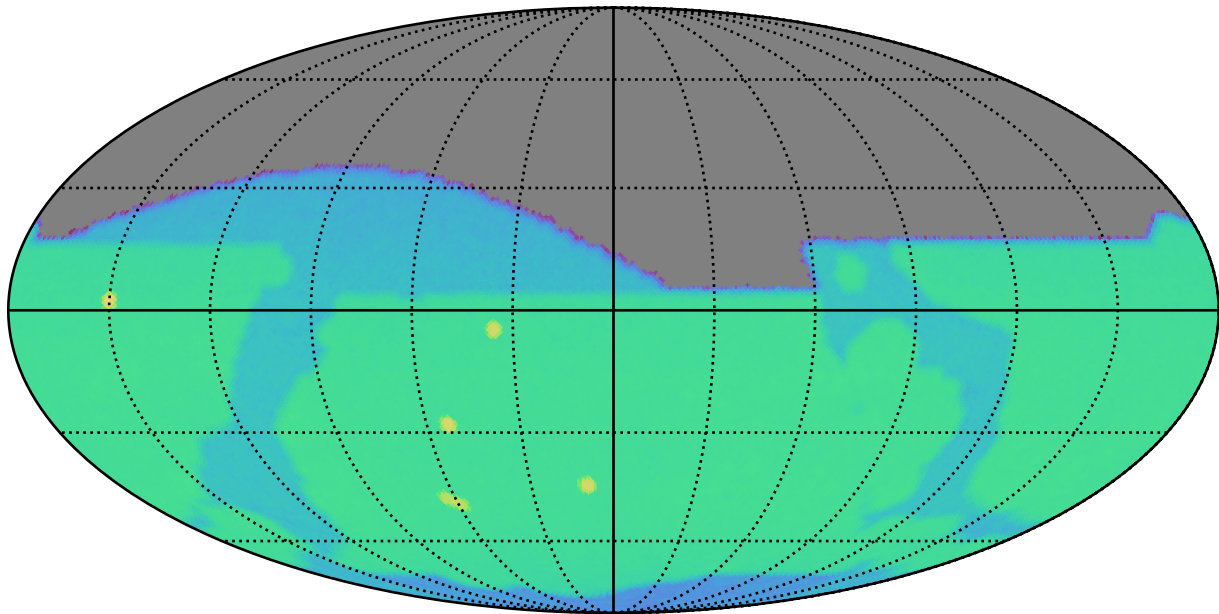
ddf_acor_sf30_lsf40_lsr10_v3.4_10yrs i: SurfaceBrightLimit
