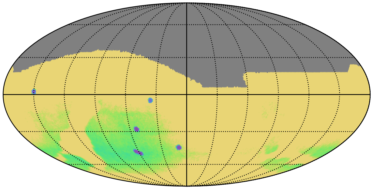
ddf_acor_sf30_lsf40_lsr10_v3.4_10yrs : Parallax Uncert @ 22.4
