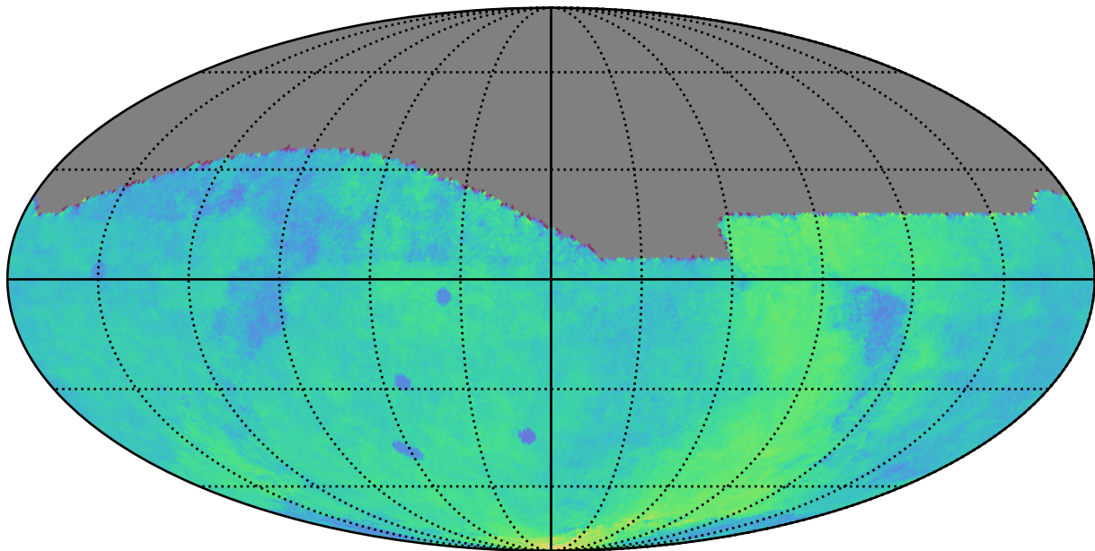
ddf_acor_sf30_lsf40_lsr10_v3.4_10yrs : Parallax Coverage @ 24.0
