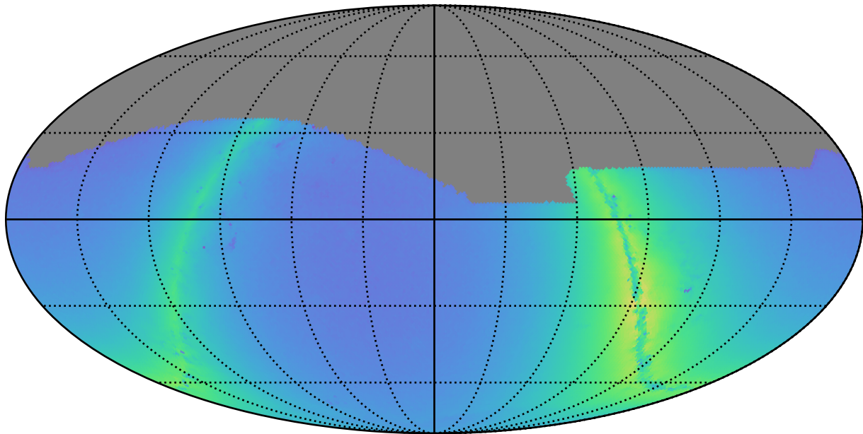
ddf_acor_sf30_lsf40_lsr10_v3.4_10yrs r: Nstars_no_crowding
