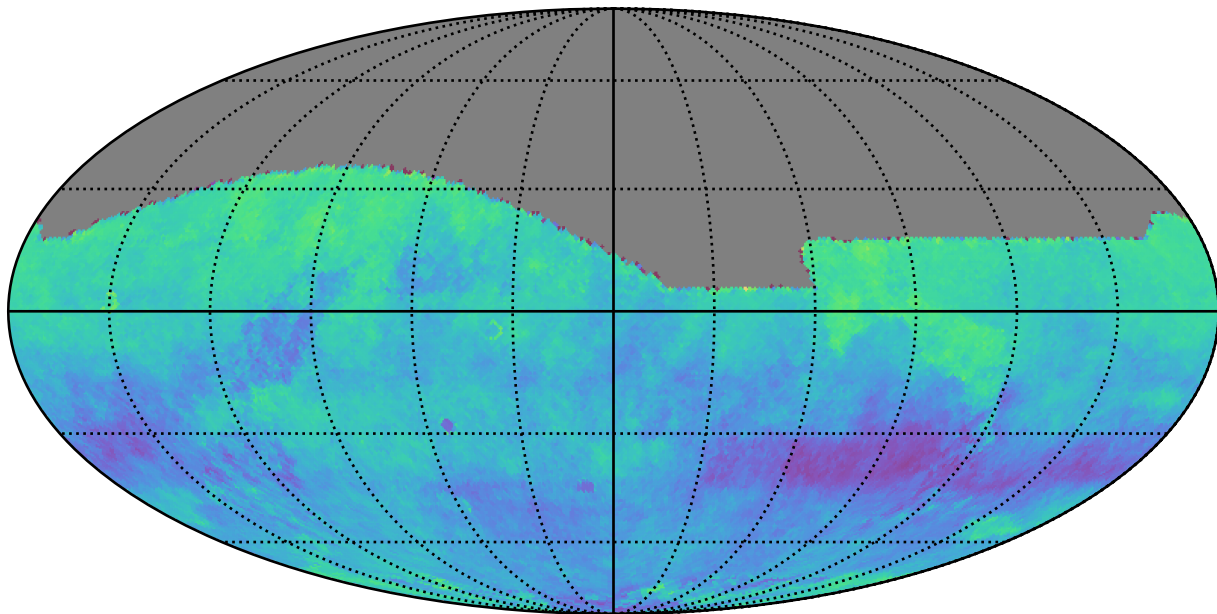
ddf_acor_sf30_lsf40_lsr10_v3.4_10yrs r: Kuiper rotSkyPos
