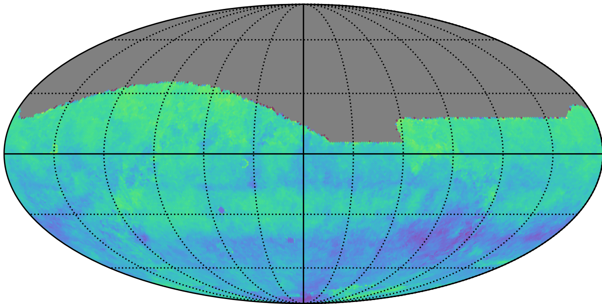
ddf_acor_sf30_lsf40_lsr10_v3.4_10yrs i: Kuiper rotSkyPos
