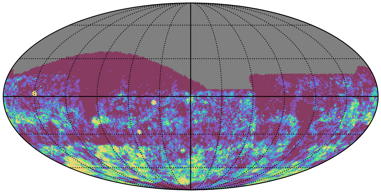
ddf_acor_sf30_lsf40_lsr10_v3.4_10yrs r band: Gaps_3hr
