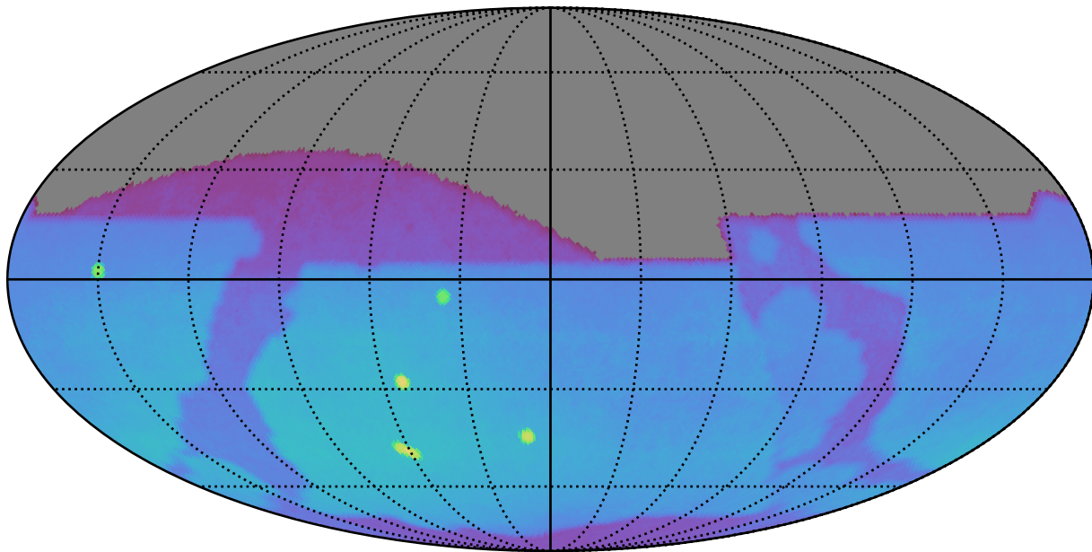
ddf_acor_sf30_lsf40_lsr10_v3.4_10yrs : Brown Dwarf, L7
