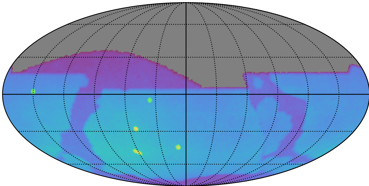
ddf_acor_sf30_lsf40_lsr10_v3.4_10yrs : Brown Dwarf, L4
