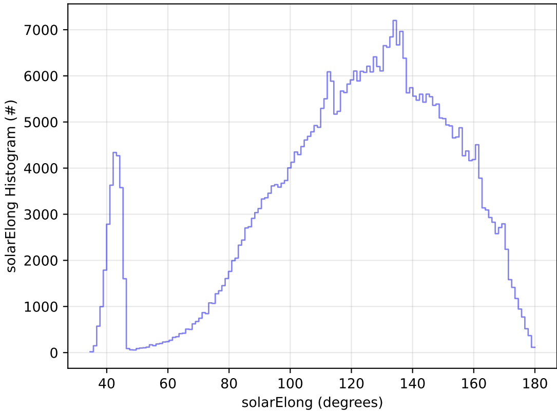
ddf_acor_sf30_lsf40_lsr10_v3.4_10yrs WFD z band: solarElong Histogram
