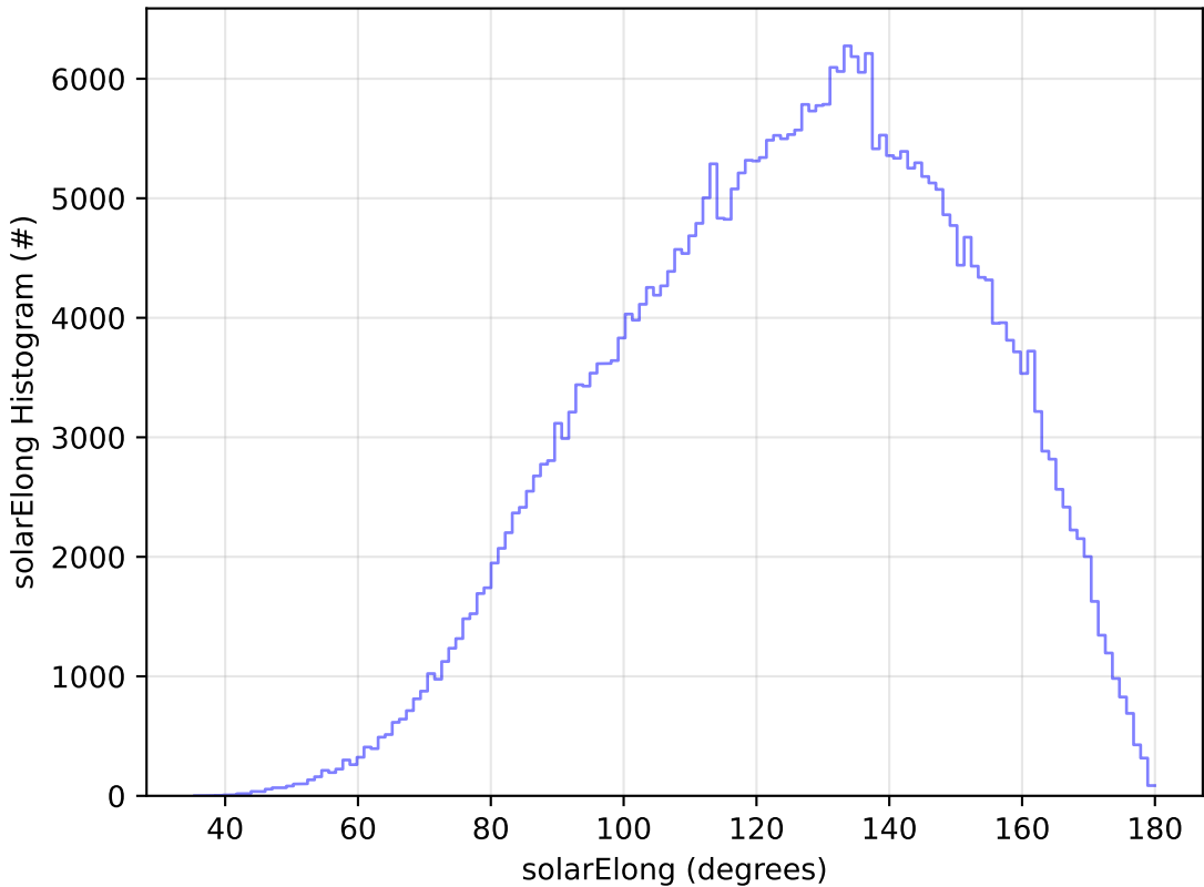
ddf_acor_sf30_lsf40_lsr10_v3.4_10yrs WFD y band: solarElong Histogram
