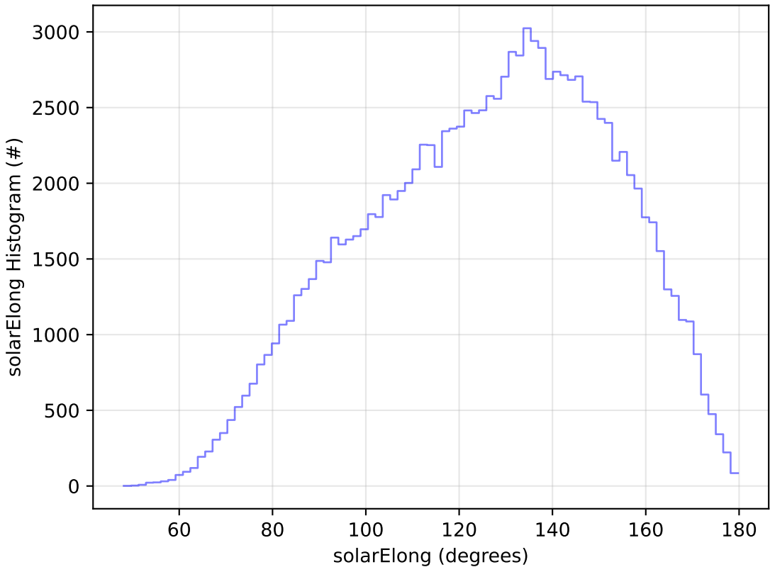
ddf_acor_sf30_lsf40_lsr10_v3.4_10yrs WFD u band: solarElong Histogram
