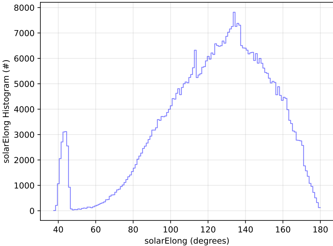
ddf_acor_sf30_lsf40_lsr10_v3.4_10yrs WFD r band: solarElong Histogram
