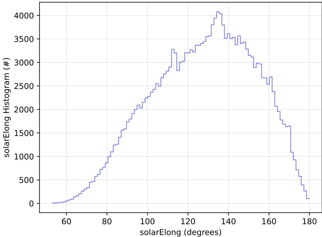
ddf_acor_sf30_lsf40_lsr10_v3.4_10yrs WFD g band: solarElong Histogram
