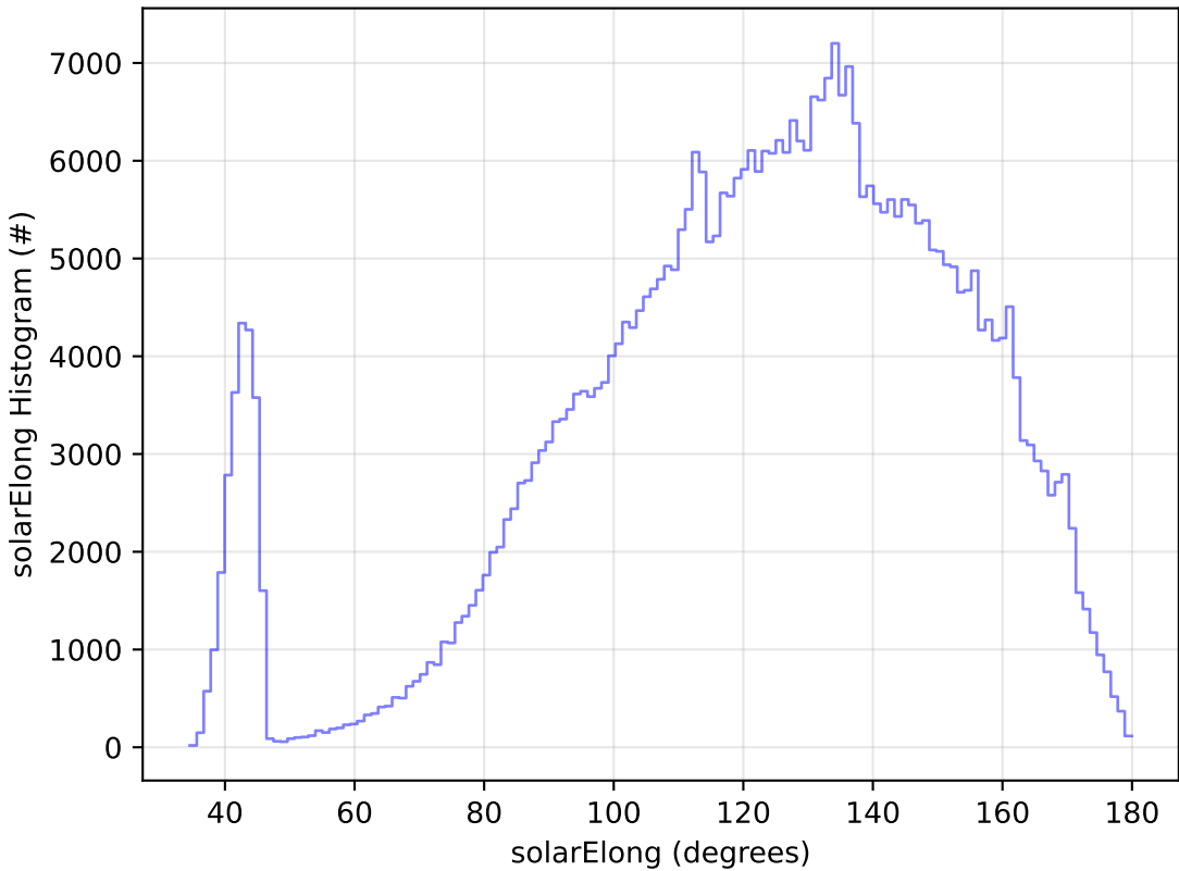
ddf_acor_sf30_lsf40_lsr10_v3.4_10yrs All sky z band: solarElong Histogram
