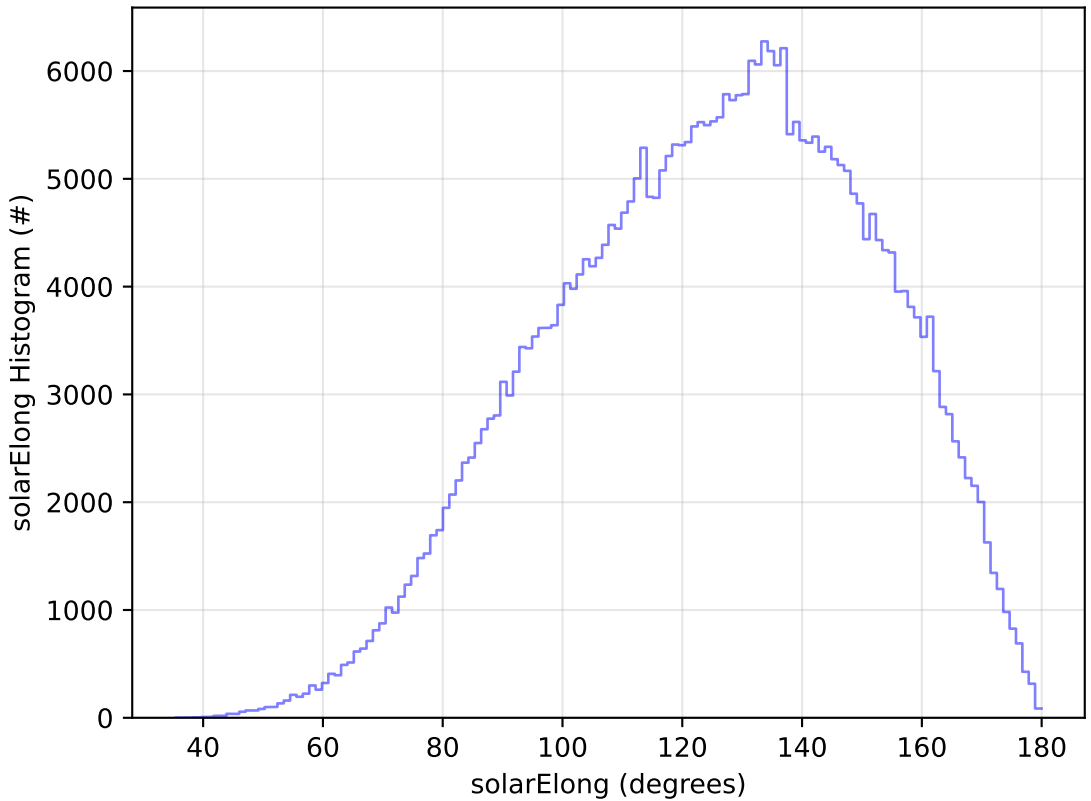
ddf_acor_sf30_lsf40_lsr10_v3.4_10yrs All sky y band: solarElong Histogram
