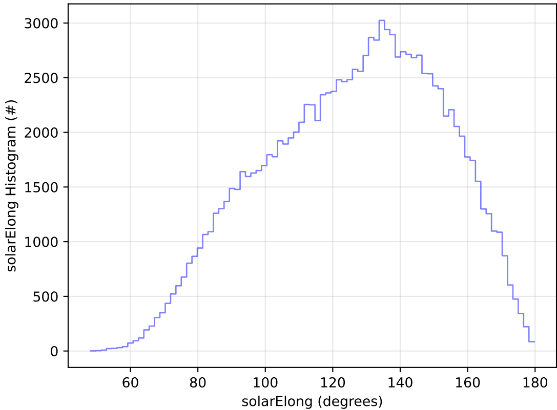
ddf_acor_sf30_lsf40_lsr10_v3.4_10yrs All sky u band: solarElong Histogram
