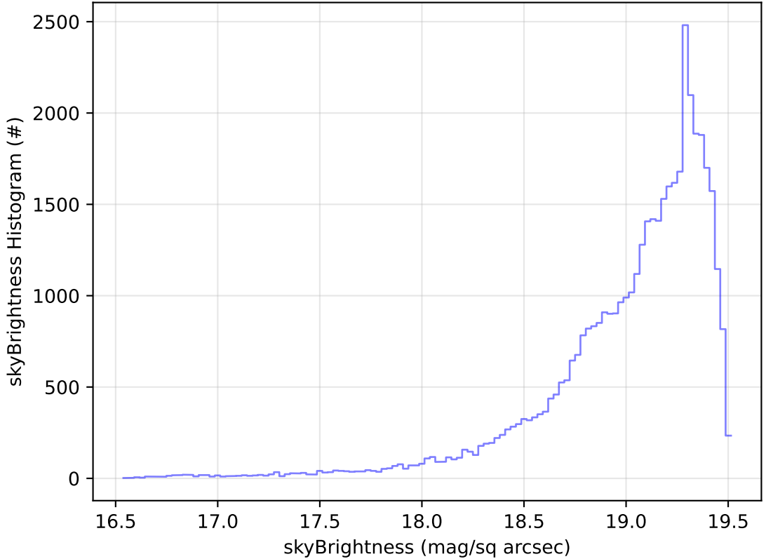
ddf_acor_sf30_lsf40_lsr10_v3.4_10yrs Yr 1 z band: skyBrightness Histogram
