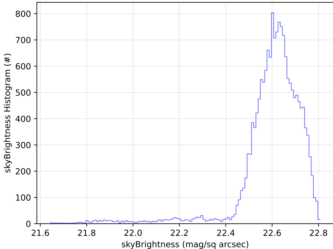
ddf_acor_sf30_lsf40_lsr10_v3.4_10yrs Yr 1 u band: skyBrightness Histogram
