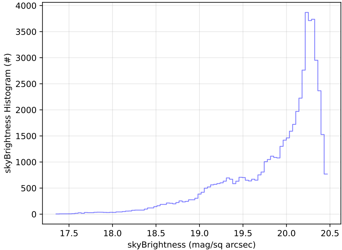
ddf_acor_sf30_Isf40_Isr10_v3.4_10yrs Yr 1 i band: skyBrightness Histogram
