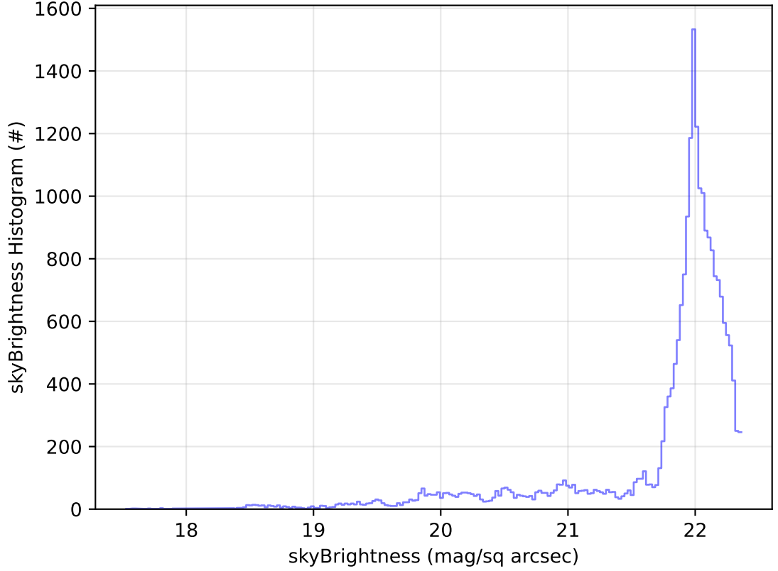
ddf_acor_sf30_lsf40_lsr10_v3.4_10yrs Yr 1 g band: skyBrightness Histogram
