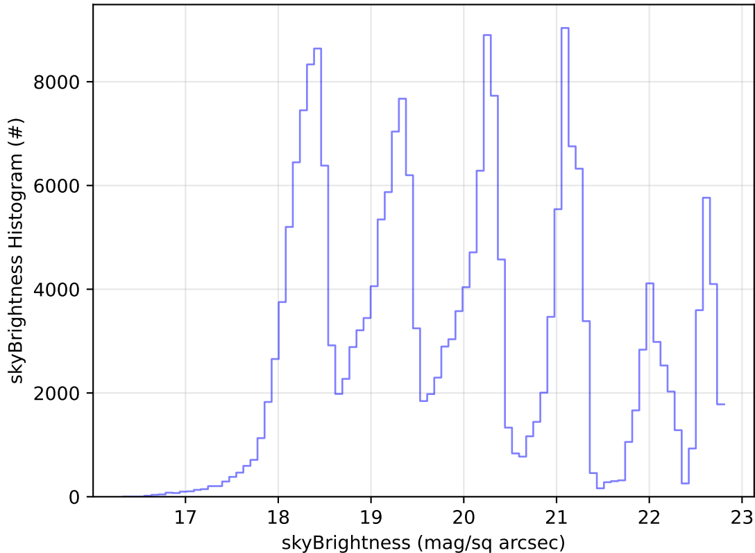
ddf_acor_sf30_lsf40_lsr10_v3.4_10yrs Yr 1 all bands: skyBrightness Histogram
